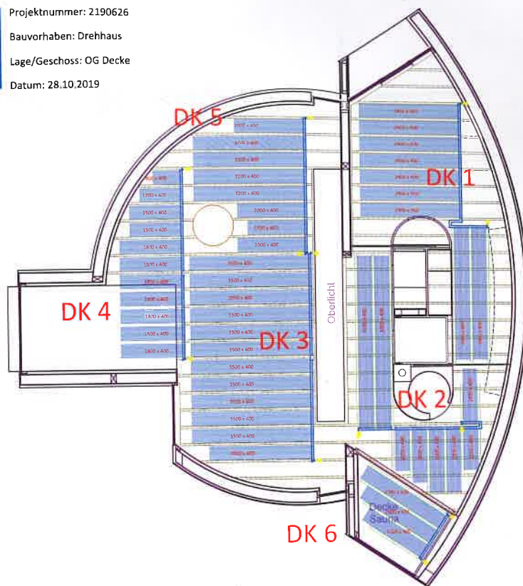
BioClina Deckenplan
